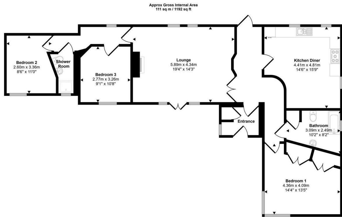
Floorplan
